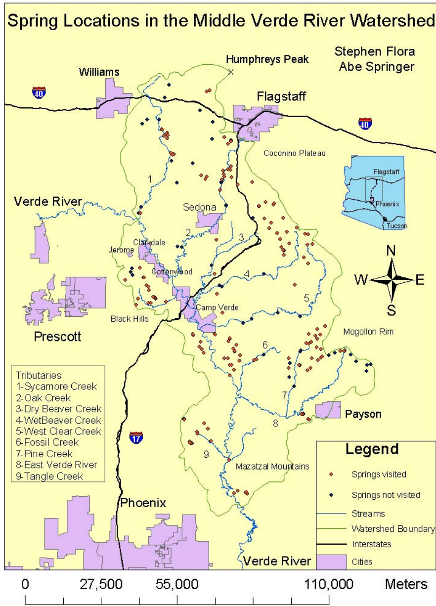
Figure 1 – GIS Map of springs from Phase I of Middle Verde River Watershed springs monitoring study.
