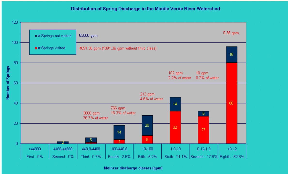
Figure 2 – Distribution of spring discharges measured in Phase I of the Verde Springs monitoring study.
