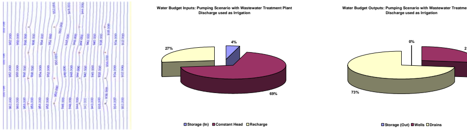
Figure 6. Water table elevation (left), water budget inputs (middle), and water budget outputs (right) in the groundwater model under a pumping scenario with wastewater treatment plant effluent being used to irrigate
