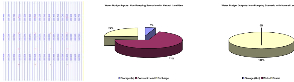
Figure 4. Water table elevation (left), water budget inputs (middle), and water budget outputs (right) in the groundwater model under natural conditions (i.e. no pumping, irrigation or impervious surfaces).
