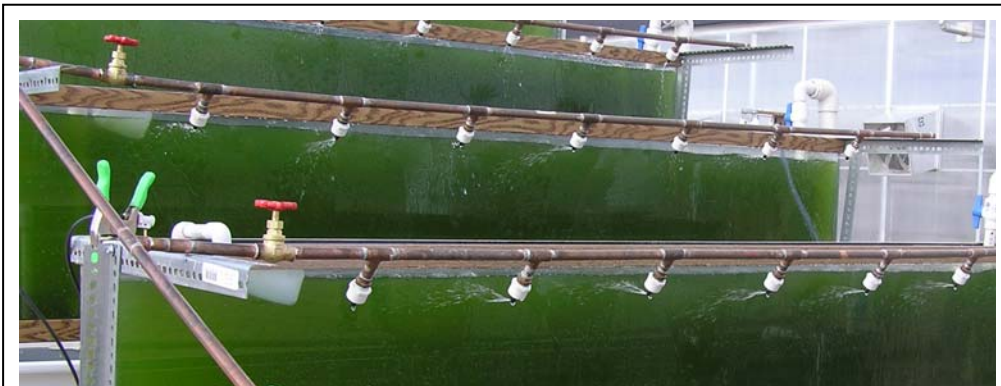
Figure 9. A evaporative cooling system for culture temperature control.
